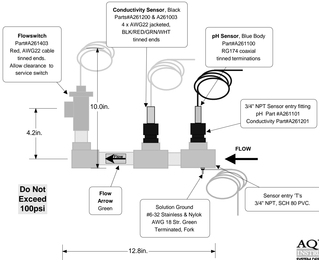
Drawing: Hdr_CP_F
